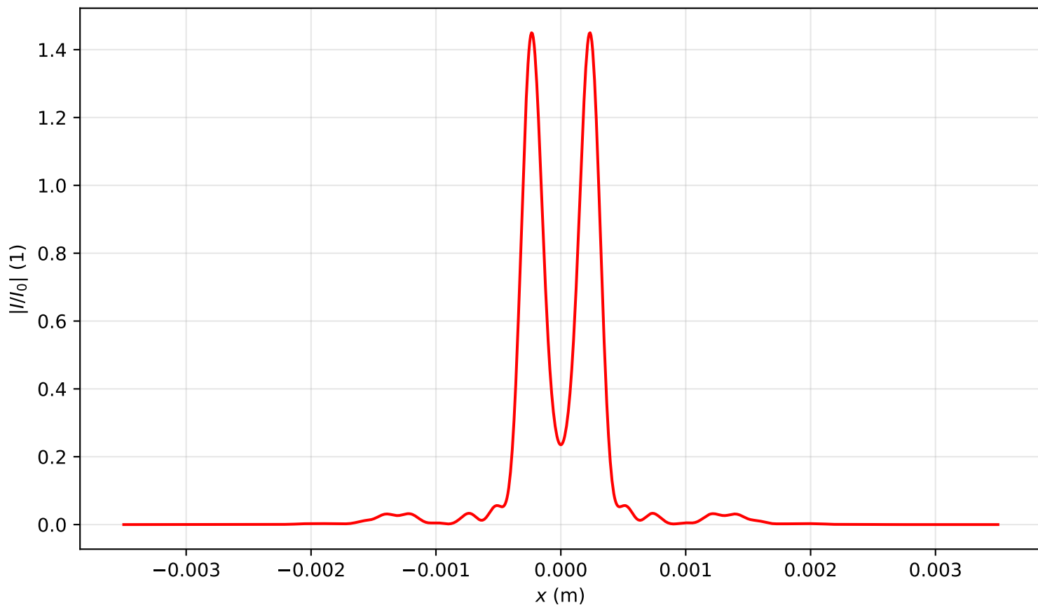
Intensity profile I(x, y = 0, z = 1.911)/I_0 , P_{in}=3.0P_{cr} , artificial time
